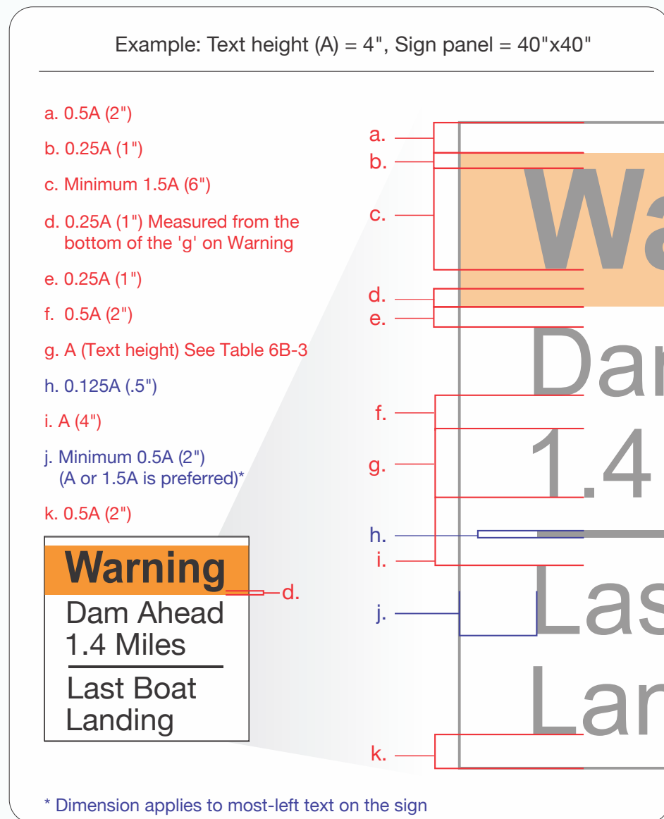
Figure 6B-8 "Last Landing Above (On-Water) Sign" Face Dimensions
